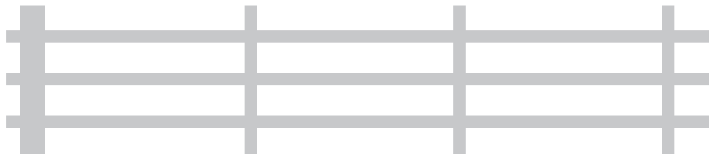
MAX-FLOW 68% OPEN SLOTS 1/4" X 1-1/2", IN ROWS ACROSS WIDTH OF SHEET. VERTICAL BARS 3/32" WIDE, WITH EVERY THIRD BAR 3/16"
